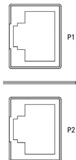
PROFINET IO 总线适配器的引脚分配 2×RJ45
